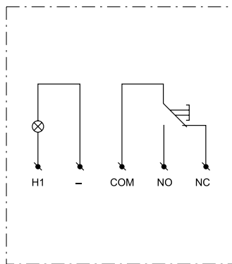
Pienjännitepainike PS1
