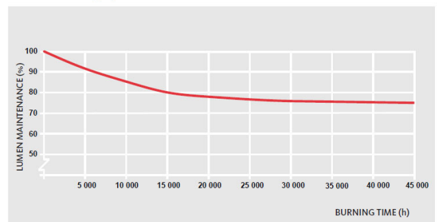
Lumen maintenance Aura Crystal TT Long Life 12 h switching cycle (11 h on, 1 h off)
