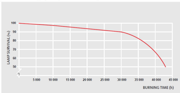
Lifetime Aura Crystal TT Long Life 12 h switching cycle (11 h on, 1 h off)
