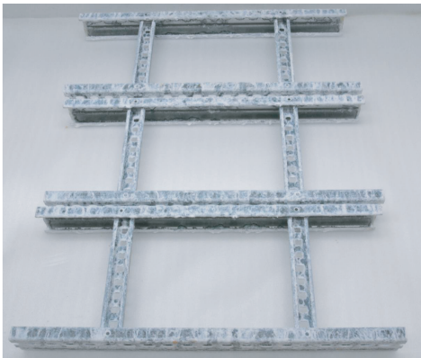
After 1000 h white rust has occurred on the Z4 cable ladders, it does not affect function or service life.
