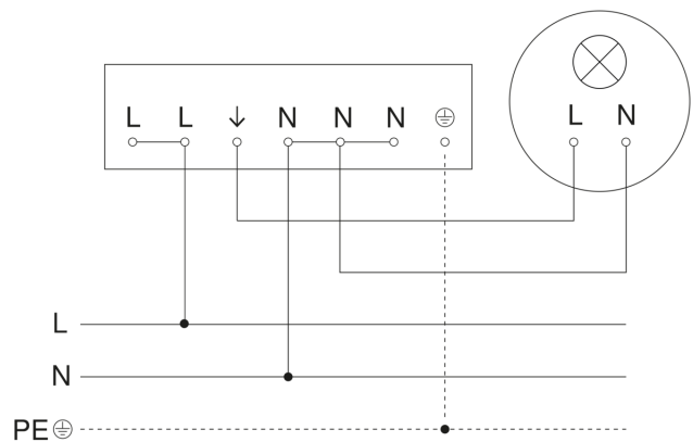
Master circuit diagram
