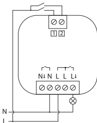
1-pole switching of live (L)
