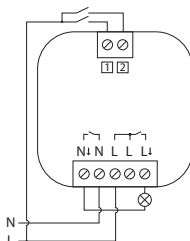
2-pole switching of phase (L) and zero (N)
