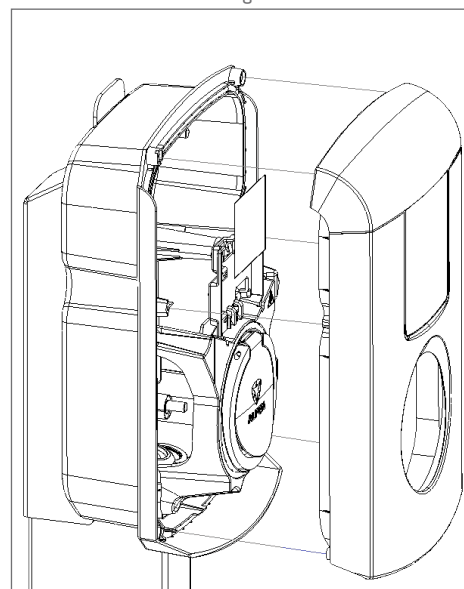
Fix the front cover back onto the charging station with the included bolts.
