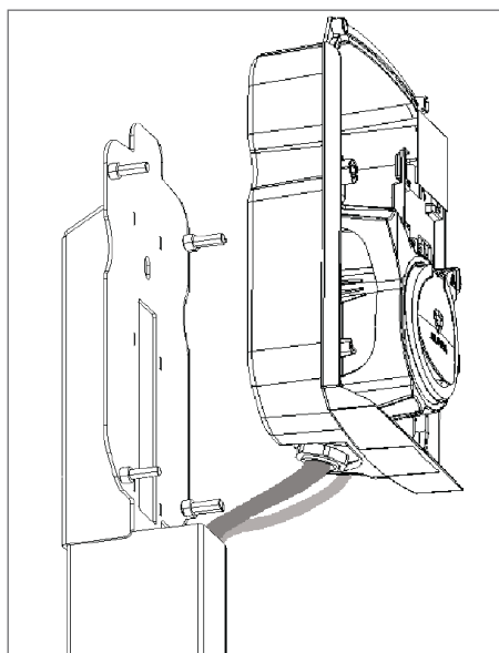
Connect the wires according to the instructions of the Eve Single S- or Pro-line manual.
