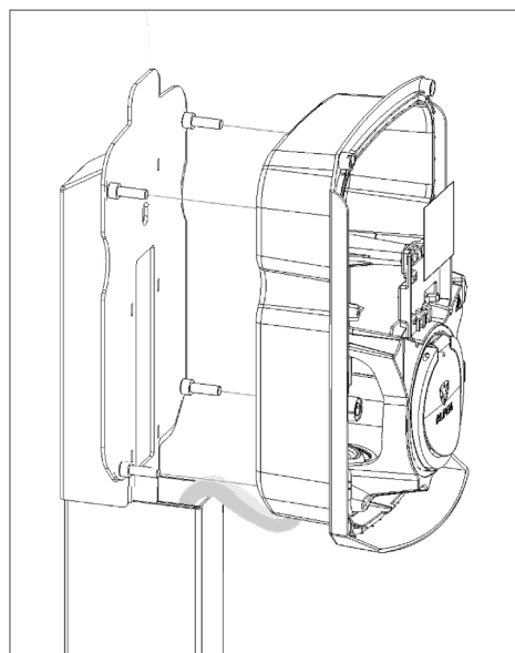
Fix the charging station in place with the included M8 washers and nuts.
