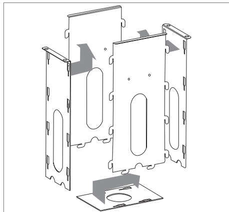
3. Attach all the narrow to the wide parts first. Attach the bottom plate last. Apply masking tape over the threaded holes to prevent dirt from entering.
