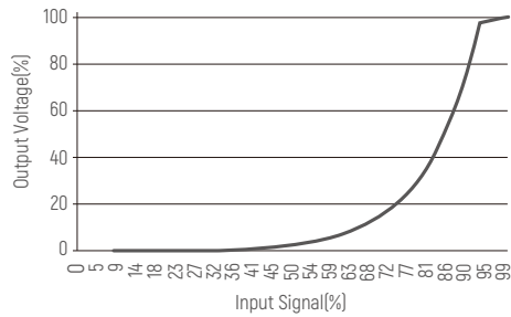
0/1-10V Curve
