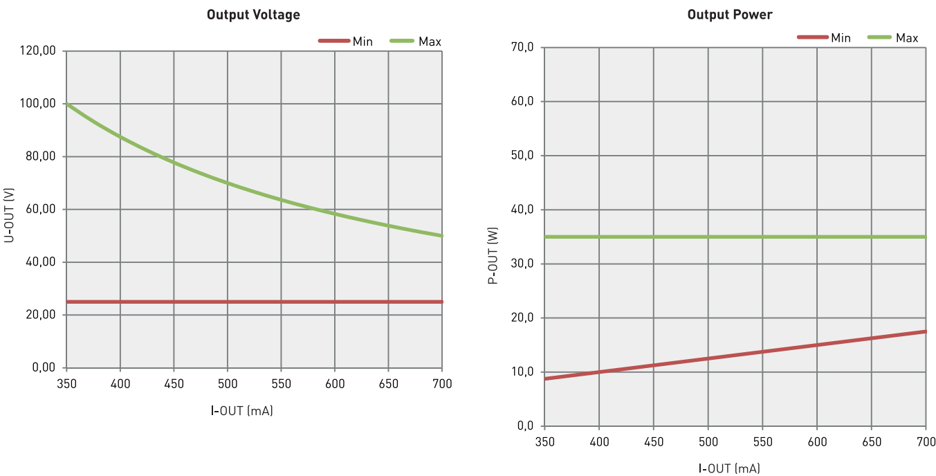
Current setting resistor values LL35/2-E-DA-iC
