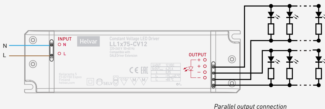
Parallel output connection
