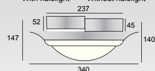
Astro & Cosmo High 340 With halolight Without halolight
