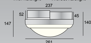
Astro & Cosmo High 300 With halolight Without halolight
