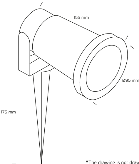
*The drawing is not drawn to scale
