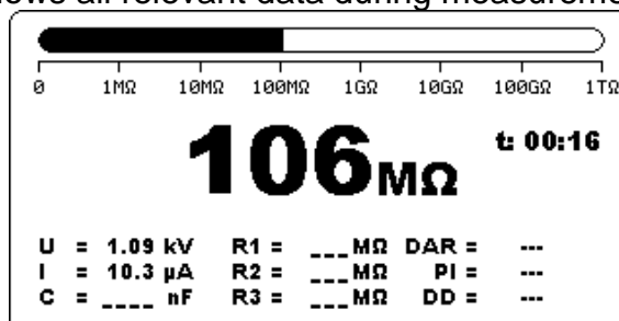
Figure 3.7: Measurement window
