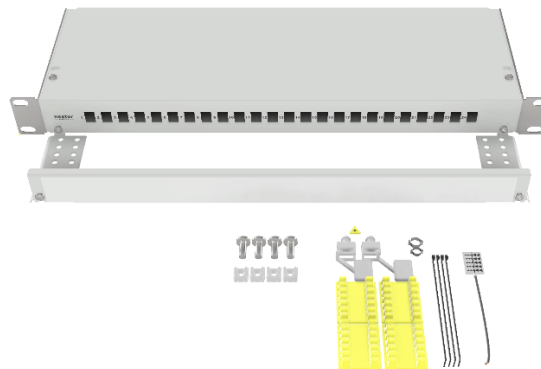
Nestor Panel Plus basic assembly for SC-S adapters (LV2595)
