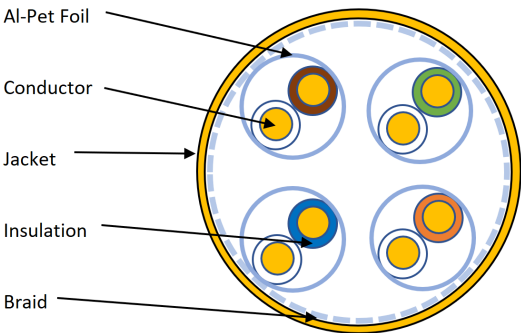
Cross-section diagram
