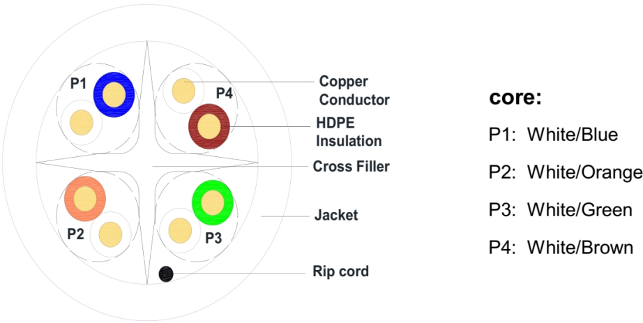
Cross-section diagram
